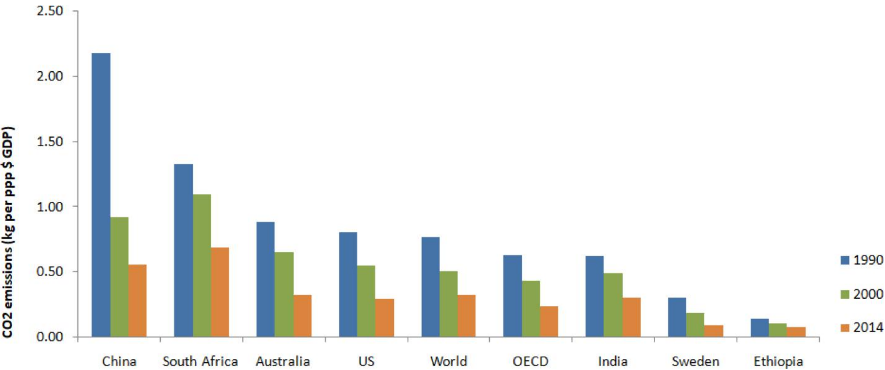
Figure 8: Carbon dioxide emissions per unit GDP in selected countries and regions. Source: Carbon Dioxide Information Analysis Center, Environmental Sciences Division, Oak Ridge National Laboratory, Tennessee, United States.
